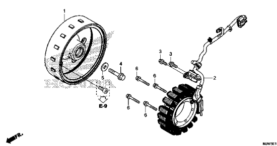
GENERATOR
