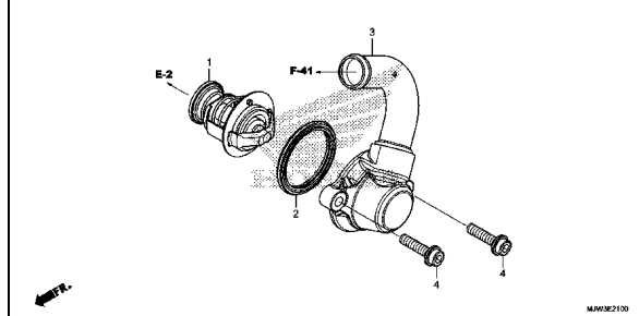
THERMOSTAT
