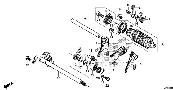
GEARSHIFT DRUM
