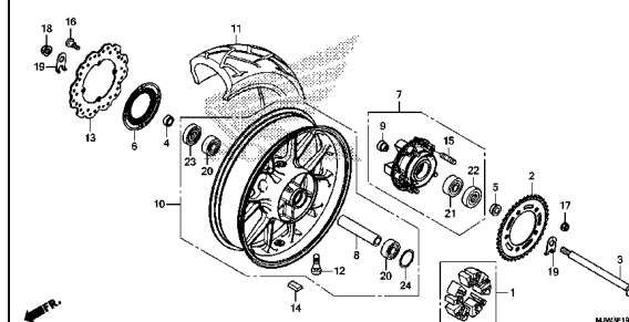
REAR WHEEL
