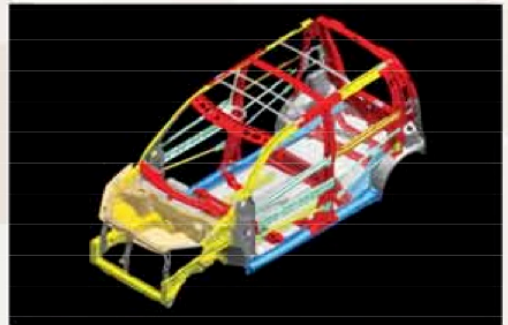
Energy absorbing body structure for safer drives
